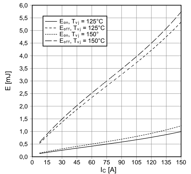
Schaltverluste IGBT-Wechselr. (typisch) switching losses IGBT-inverter (typical) E_{on} = f(I_C) , E_{off} = f(I_C) V_{GE} = \pm 15\text{ V} , R_{Gon} = 5,1\ \Omega , R_{Goff} = 5,1\ \Omega , V_{CE} = 300\text{ V}
