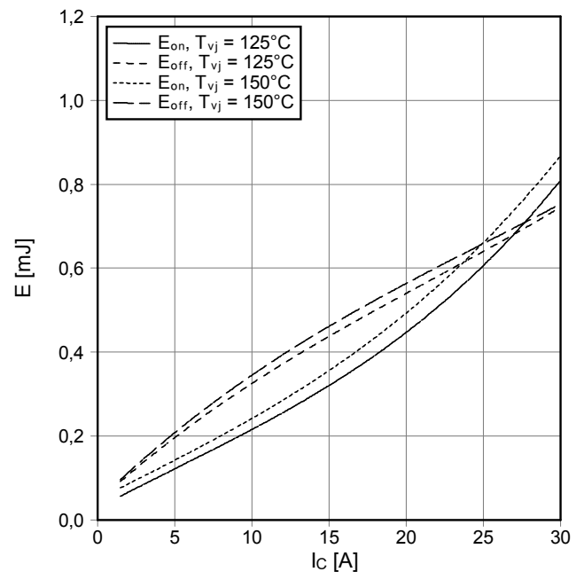
Schaltverluste IGBT-Wechselr. (typisch) switching losses IGBT-inverter (typical) E_{on} = f(I_C), E_{off} = f(I_C) V_{GE} = \pm 15 \text{ V}, R_{Gon} = 22 \Omega, R_{Goff} = 22 \Omega, V_{CE} = 300 \text{ V}
