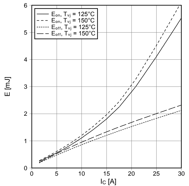
Schaltverluste IGBT-Wechselr. (typisch) switching losses IGBT-inverter (typical) E_{on} = f(I_C), E_{off} = f(I_C) V_{GE} = \pm 15\text{ V}, R_{Gon} = 39\ \Omega, R_{Goff} = 39\ \Omega, V_{CE} = 600\text{ V}
