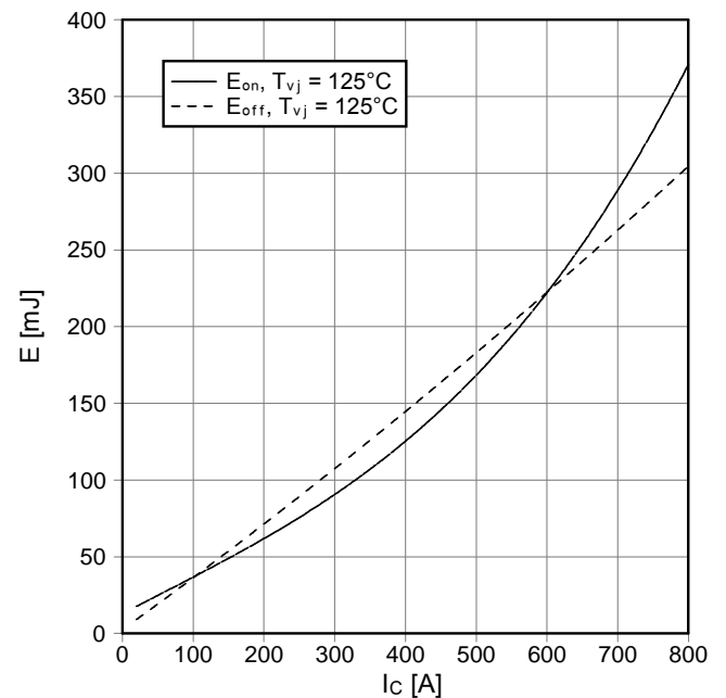
Schaltverluste IGBT-Wechselr. (typisch) switching losses IGBT-inverter (typical) E_{on} = f(I_c) , E_{off} = f(I_c) V_{GE} = \pm 15\text{ V} , R_{Gon} = 3,6\ \Omega , R_{Goff} = 4,4\ \Omega , V_{CE} = 900\text{ V}
