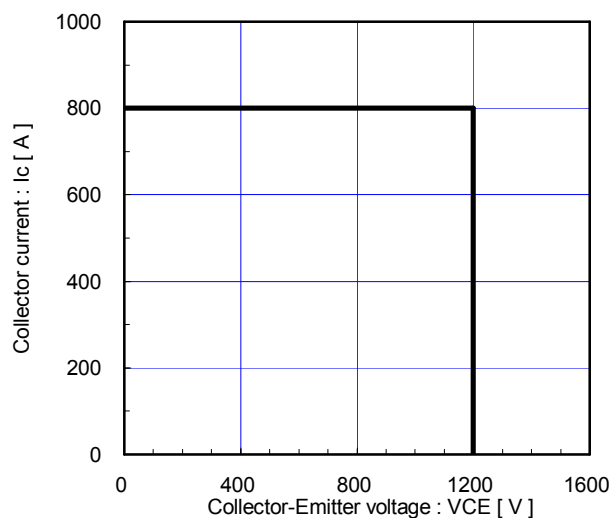
Reverse bias safe operating area (max.) +V_{GE}=15V, -V_{GE} \leq 15V, R_G \geq 1.5\Omega, T_j \leq 125^\circ C
