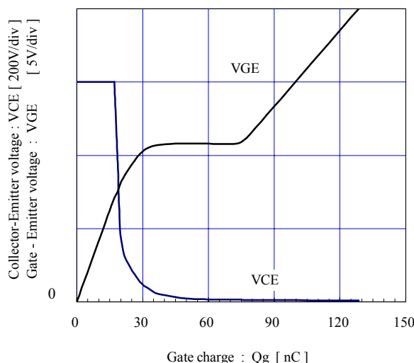
[ Inverter ] Dynamic Gate charge (typ.) Vcc=600V, Ic=35A, Tj= 25°C
