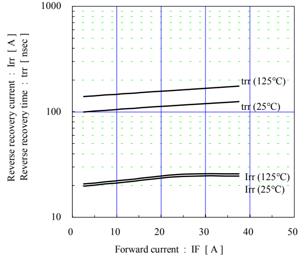
[ Inverter ] Reverse recovery characteristics (typ.) Vcc=600V, VGE=±15V, Rg=43 Ω
