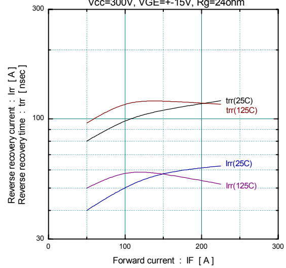
[ Inverter ] Reverse recovery characteristics (typ.) Vcc=300V, VGE=+-15V, Rg=24ohm
