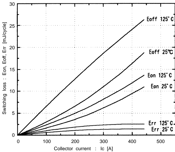
Switching loss vs. Collector current Vcc=300V, RG=6.8 ohm, VGE=±15V
