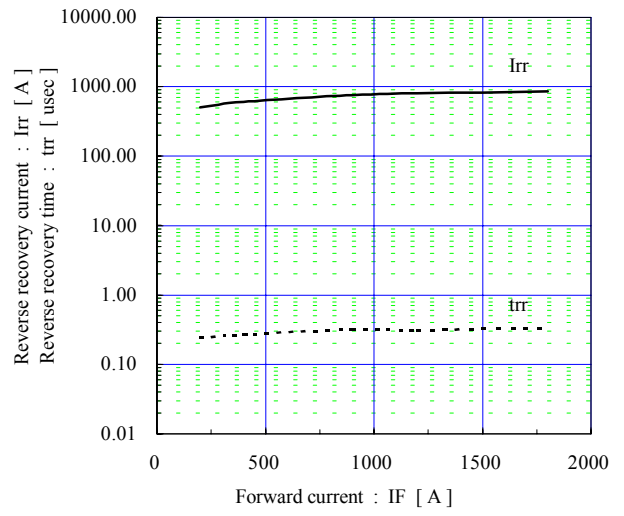
Reverse recovery characteristics (typ.) Vcc=600V, VGE=±15V, Rgon=1.8Ω, Tj=125°C
