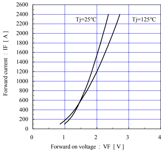
Forward current vs. Forward on voltage (typ.) sense terminal
