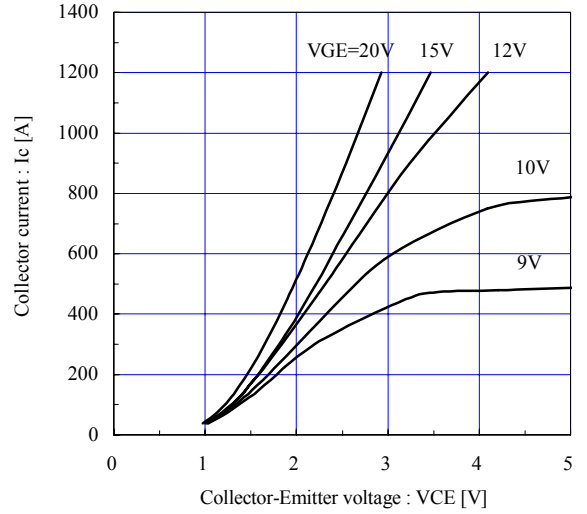
Collector current vs. Collector-Emitter voltage (typ.) T_j=125^\circ C , sense terminal
