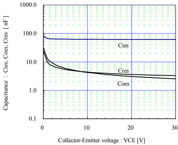
Capacitance vs. Collector-Emitter voltage (typ.) V_{GE}=0V , f=1MHz , T_j=25^\circ C
