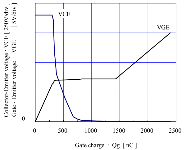
Dynamic Gate charge (typ.) T_j=25^\circ C
