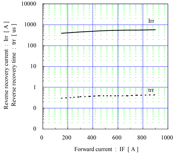
Reverse recovery characteristics (typ.) V_{cc}=900\text{V} , V_{GE}=\pm 15\text{V} , R_g=1.8\Omega , T_j=125^\circ\text{C}
