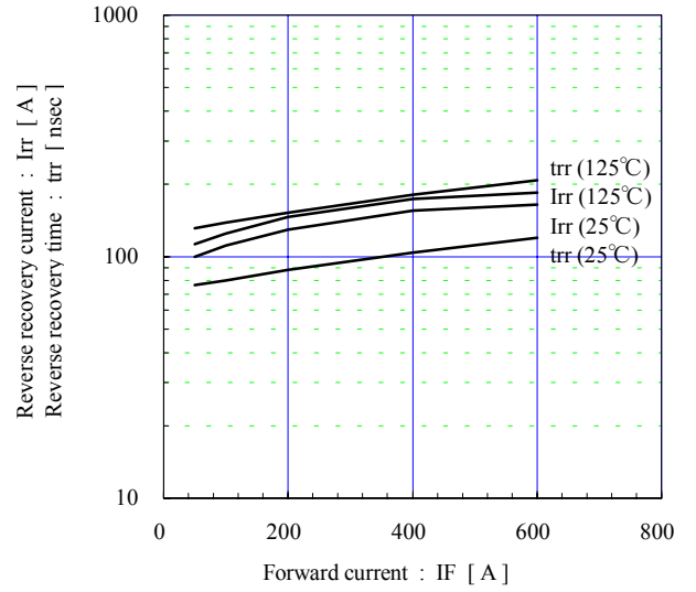
Reverse recovery characteristics (typ.) Vcc=300V, VGE=±15V, Rg=6.8Ω
