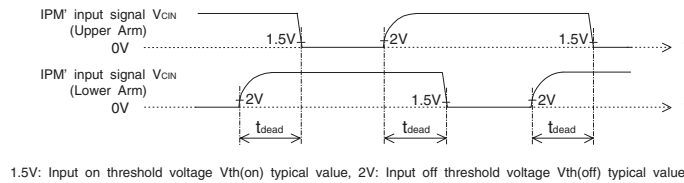
1.5V: Input on threshold voltage V_{th(on)} typical value, 2V: Input off threshold voltage V_{th(off)} typical value
