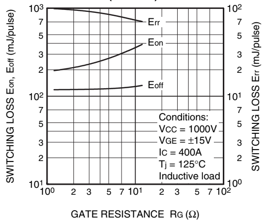
SWITCHING LOSS vs. GATE RESISTANCE (TYPICAL)
