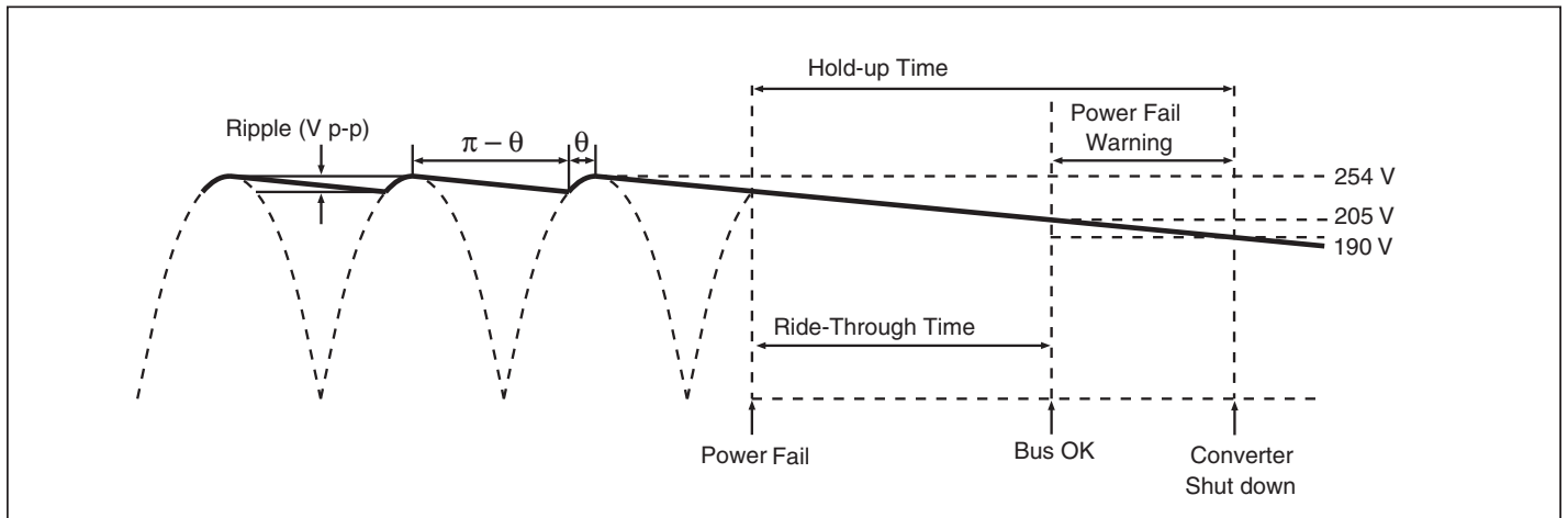
Figure 15 — Hold-up time
